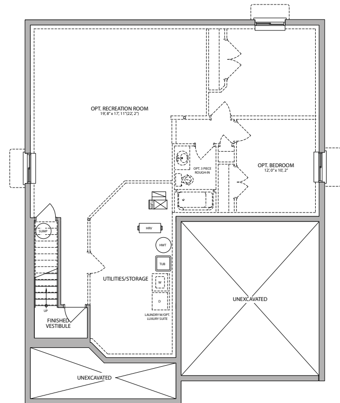
BASEMENT FLOOR PLAN Elevation A & B
